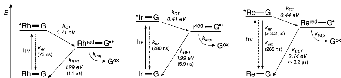
Figure 7. Proposed model for the DNA-mediated oxidation of guanine by metallointercalating photooxidants. Conjugates are represented as M—G, where the thickness of the line connecting M and G represents the extent of coupling between the metal complex and the base stack. Wavy arrows represent nonradiative decay from the excited state (*Rh, *Ir, or *Re). Reduced metal complex states are represented as M red . The guanine radical cation (G •+ ) is distinguished from permanent guanine oxidation products (G ox ). Energy level differences are to scale. Thermodynamic driving forces are shown for charge injection and BET, and lifetimes are shown in parentheses. In each scheme, the equilibrium with the poorly coupled system is omitted for clarity.
