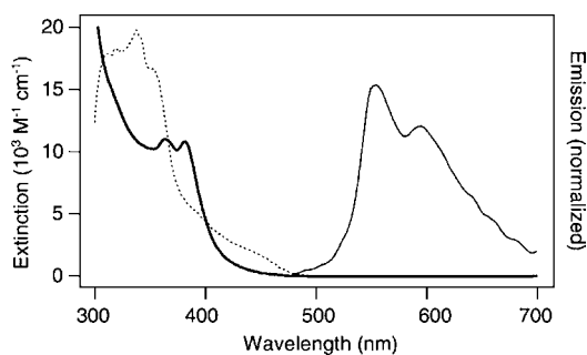
Figure 2. UV/visible steady-state characteristics of [\text{Re}(\text{CO})_3(\text{dppz})(\text{py})]^+ . The absorbance spectrum (bold), emission spectrum ( \lambda_{\text{ex}} = 355 \text{ nm} ; solid), and excitation spectrum ( \lambda_{\text{em}} = 570 \text{ nm} ; dotted) of the complex ( 18 \mu\text{M} ) in degassed acetonitrile are shown.
