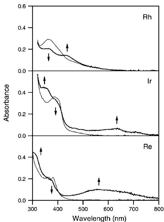
Figure 3. Steady-state UV/visible absorbance spectra of metal complexes before (thin line) and after (thick line) reduction by bulk electrolysis. Top: 16 \mu\text{M} [\text{Rh}(\text{phi})_2(\text{bpy})]^{3+} in DMF; middle: 12 \mu\text{M} [\text{Ir}(\text{ppy})_2(\text{dppz})]^+ in DMF; bottom: 20 \mu\text{M} [\text{Re}(\text{CO})_3(\text{dppz})(\text{py-OEt})]^+ in acetonitrile. Arrows indicate changes in the spectra upon reduction.
