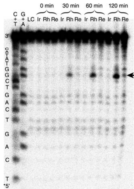
Figure 4. PAGE analysis following photooxidation of guanine by [Rh(phi) 2 (bpy')] 3+ , [Ir(ppy) 2 (dppz)] + , and [Re(CO) 3 (dppz)(py')] + covalently bound to DNA. Metal-DNA conjugates (2 \mu M in buffer: 10 mM sodium phosphate, 50 mM NaCl, pH 7.5) were irradiated for 0, 30, 60, or 120 min. DNA strand cleavage at sites of oxidation was achieved by treatment with 10% piperidine. Cleavage products were separated by 20% PAGE and visualized by phosphorimager. C+T and G+A: Maxam-Gilberts sequencing lanes; LC: light control (no metal complex); Ir, Rh, Re: the corresponding metal-DNA conjugates, irradiated for the indicated times. The DNA sequence is shown along the left edge of the gel. The position of the radiolabel is indicated by *. The 5'-G of the 5'-GG-3' doublet is indicated by an arrow.
