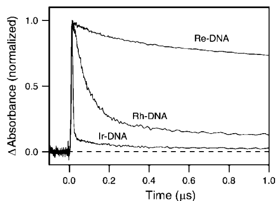
Figure 6. Transient absorption decay traces for 15 \mu M [\text{Rh}(\text{phi})_2(\text{bpy}')^{3+} (460 nm), [\text{Ir}(\text{ppy})_2(\text{dppz}')^{3+} (540 nm), and [\text{Re}(\text{CO})_3(\text{dppz})(\text{py})]^{3+} (475 nm) covalently bound to DNA following excitation at 355 nm.
